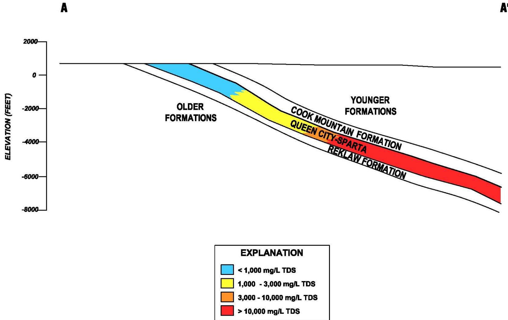
SIMPLIFIED CROSS SECTION OF THE QUEEN CITY AND SPARTA AQUIFERS WITH GENERALIZED WATER QUALITY RANGES (Modified from Baker, 1995)
