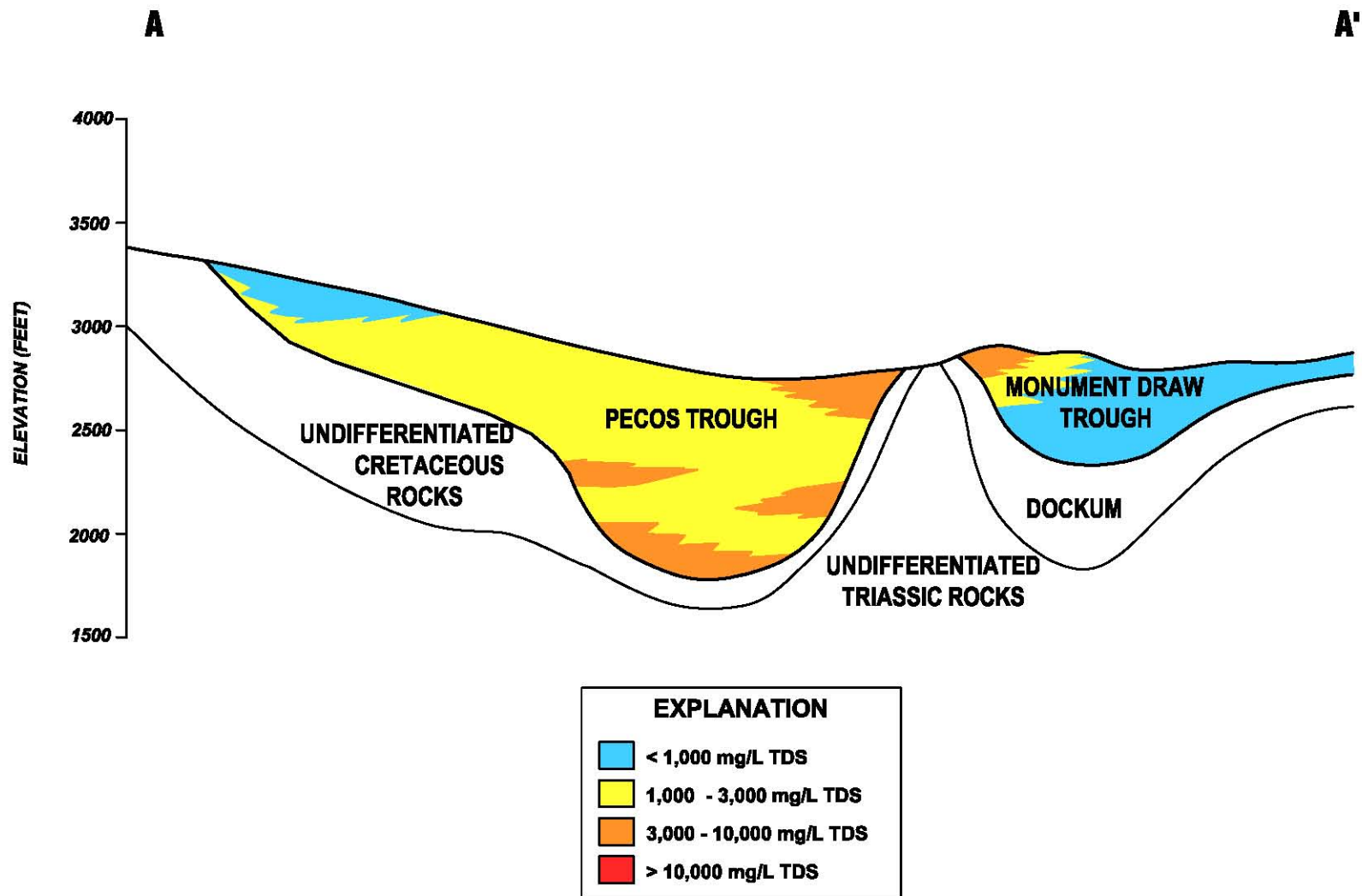
SIMPLIFIED CROSS SECTION OF THE CENOZOIC PECOS ALLUVIUM AQUIFER WITH GENERALIZED WATER QUALITY RANGES (Modified from Ashworth, 1990)
