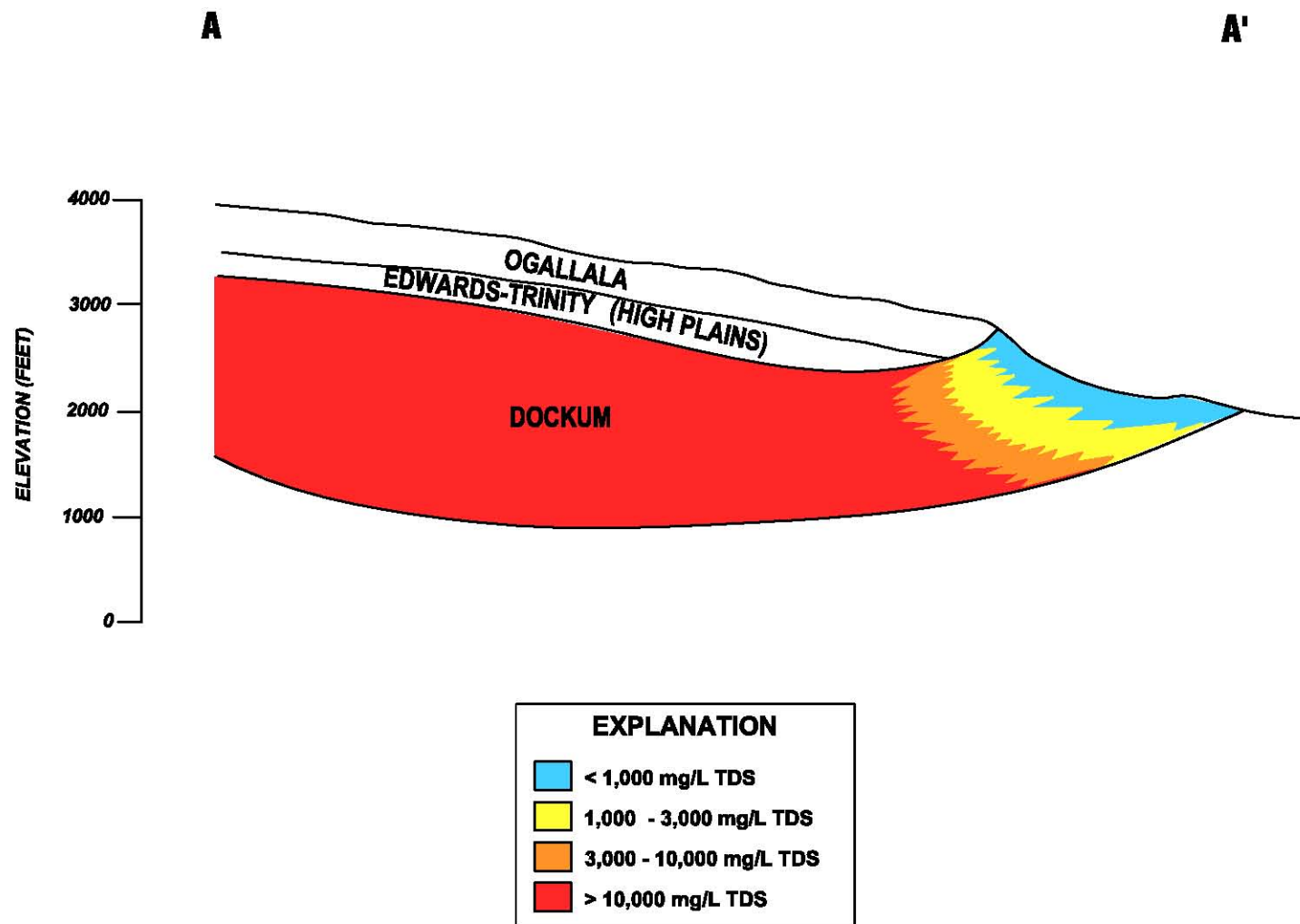
SIMPLIFIED CROSS SECTION OF THE DOCKUM AQUIFER WITH GENERALIZED WATER QUALITY RANGES (Modified from Bradley and Kalaswad, 2002)
