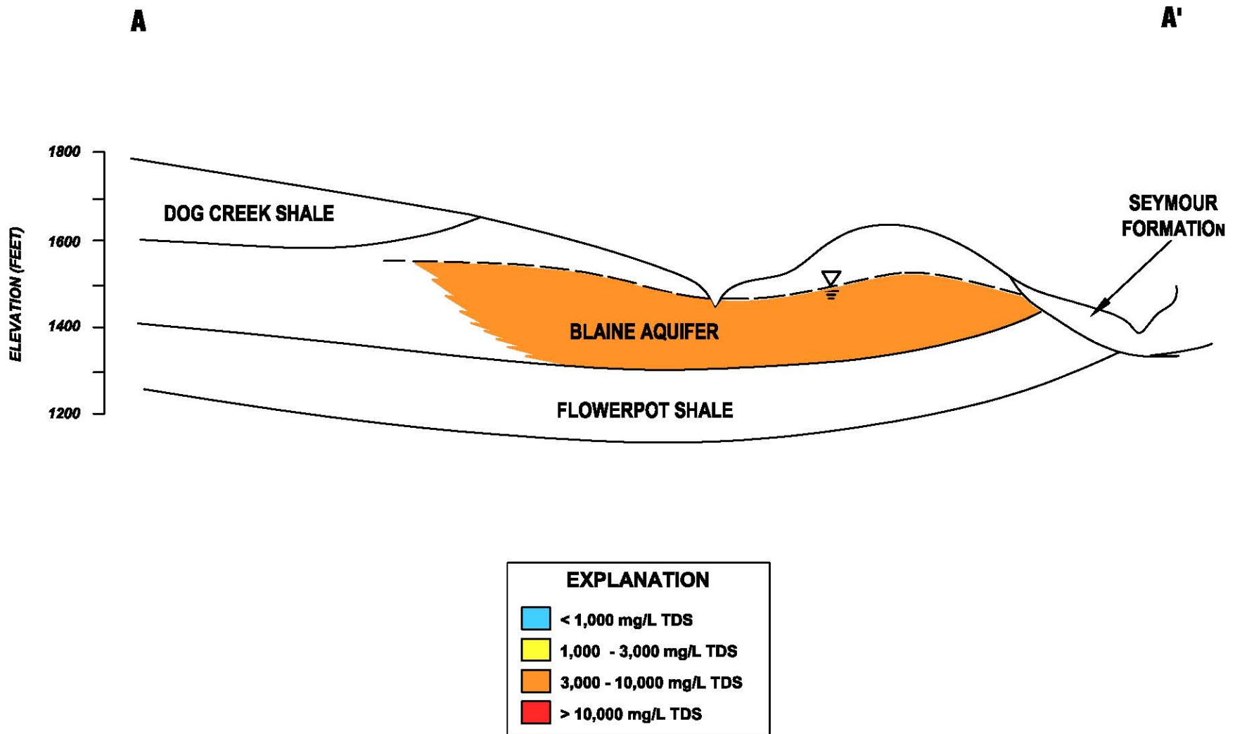
SIMPLIFIED CROSS SECTION OF THE BLAINE AQUIFER WITH GENERALIZED WATER QUALITY RANGES (Modified from Maderak, 1972)
