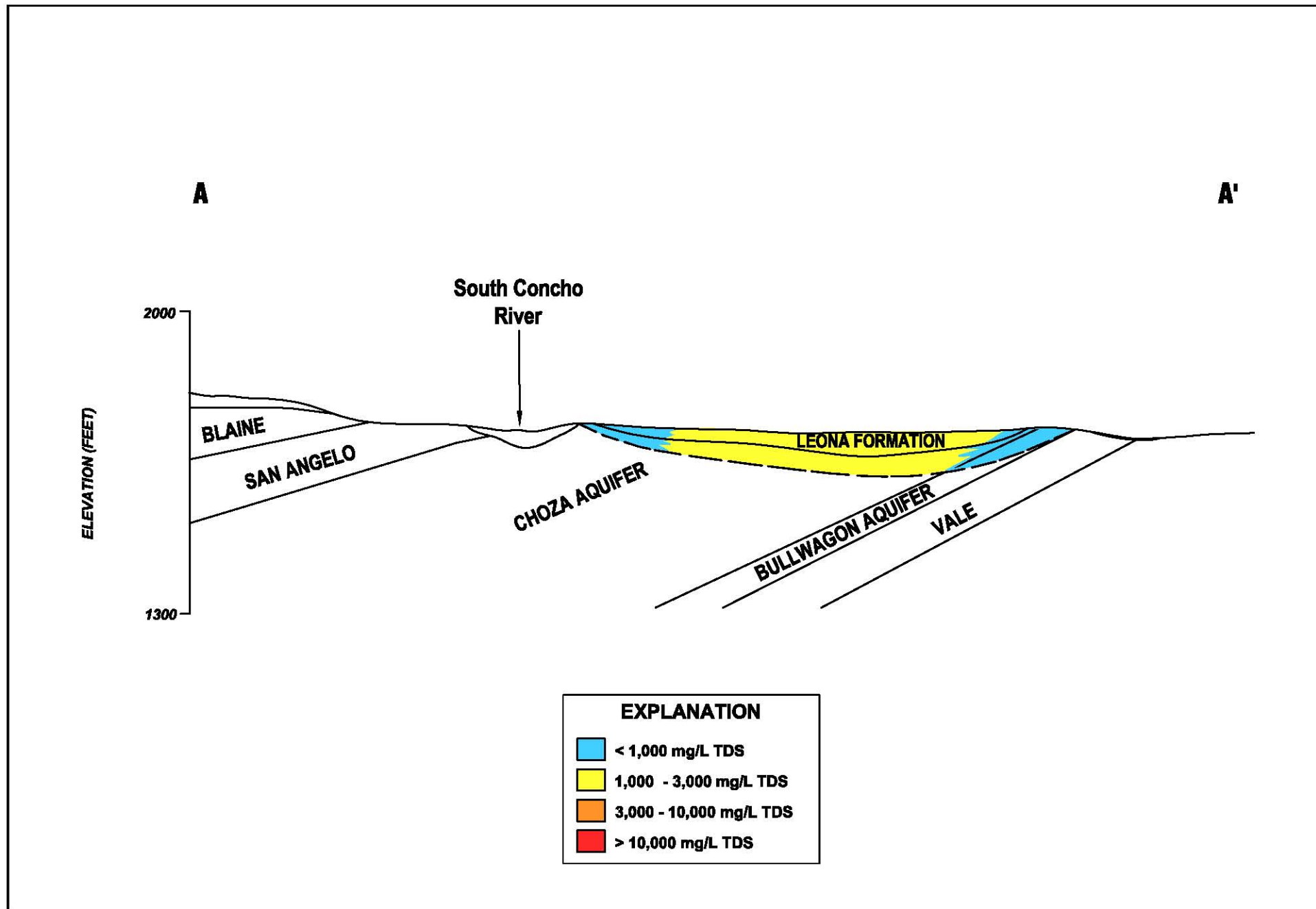
SIMPLIFIED CROSS SECTION OF THE LIPAN AQUIFER WITH GENERALIZED WATER QUALITY RANGES
