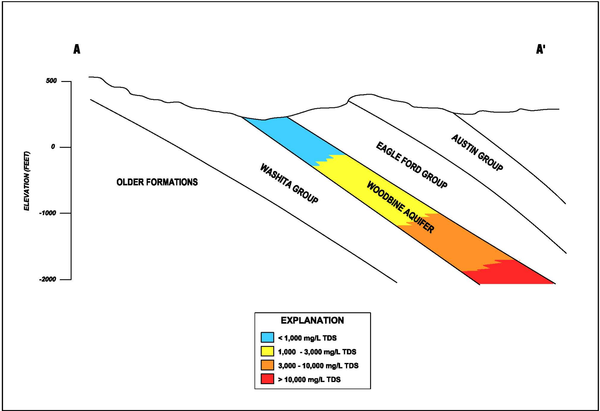
SIMPLIFIED CROSS SECTION OF THE WOODBINE AQUIFER WITH GENERALIZED WATER QUALITY RANGES (Modified from Ashworth, 1995)
