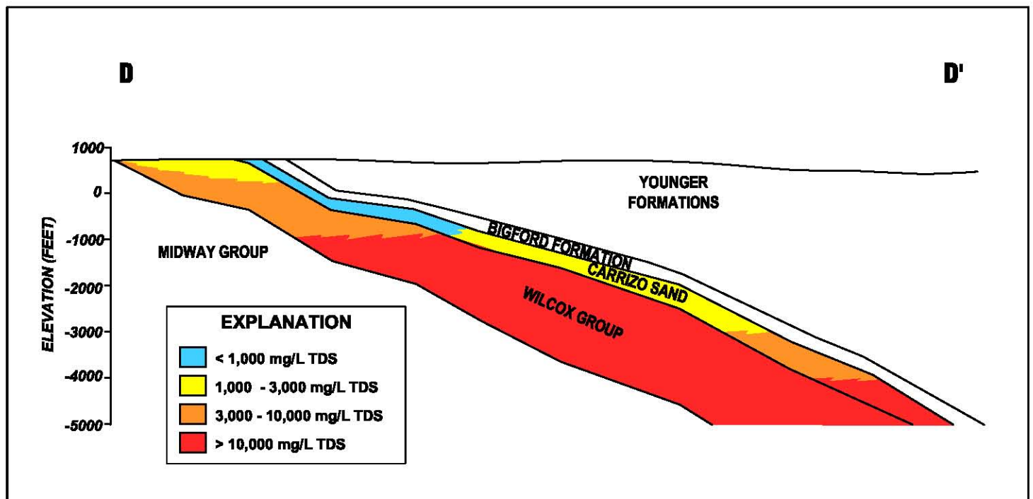
SIMPLIFIED CROSS SECTION D-D' OF THE CARRIZO-WILCOX AQUIFER WITH GENERALIZED WATER QUALITY RANGES (Modified from Baker, 1995)
