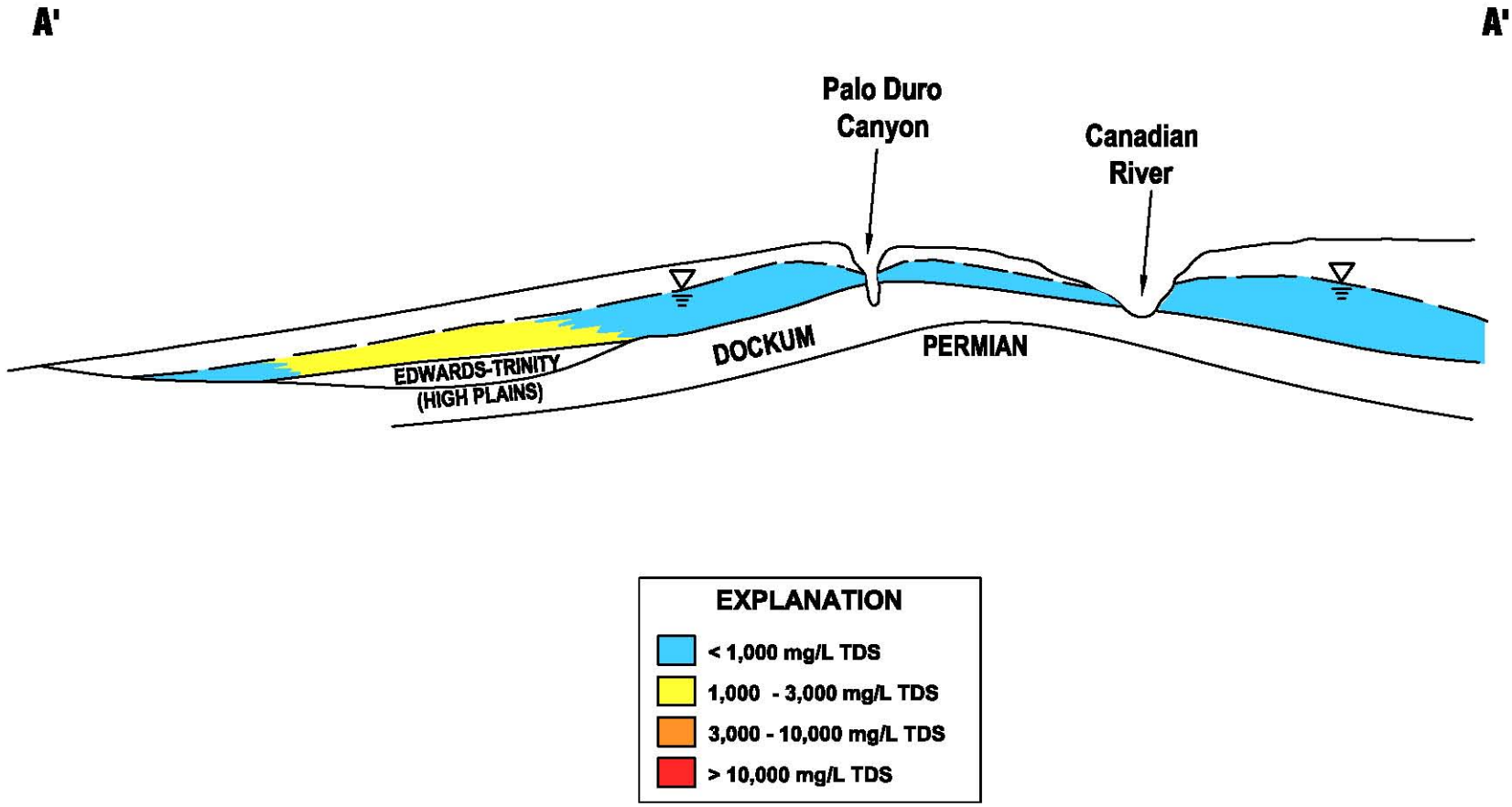
SIMPLIFIED CROSS SECTION OF THE OGALLALA AQUIFER WITH GENERALIZED WATER QUALITY RANGES (Modified from Ashworth and Hopkins, 1995)
