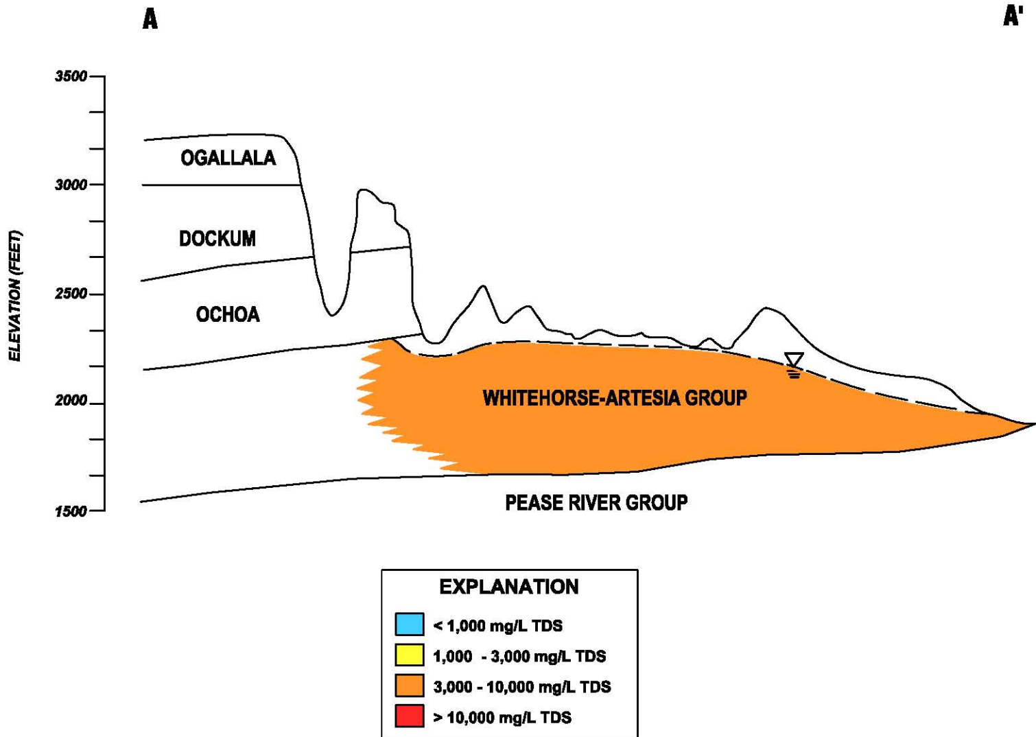
SIMPLIFIED CROSS SECTION OF THE WHITEHORSE-ARTESIA AQUIFER WITH GENERALIZED WATER QUALITY RANGES (Modified from Popkin, 1973b)
