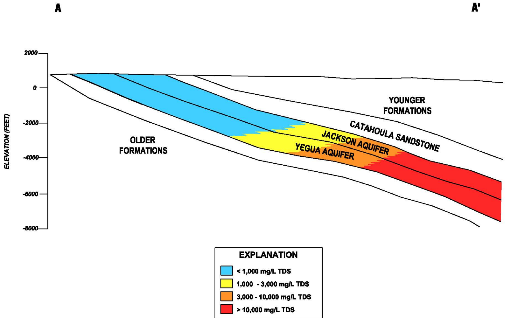
SIMPLIFIED CROSS SECTION OF THE YEGUA-JACKSON AQUIFER WITH GENERALIZED WATER QUALITY RANGES (Modified from Baker, 1995)
