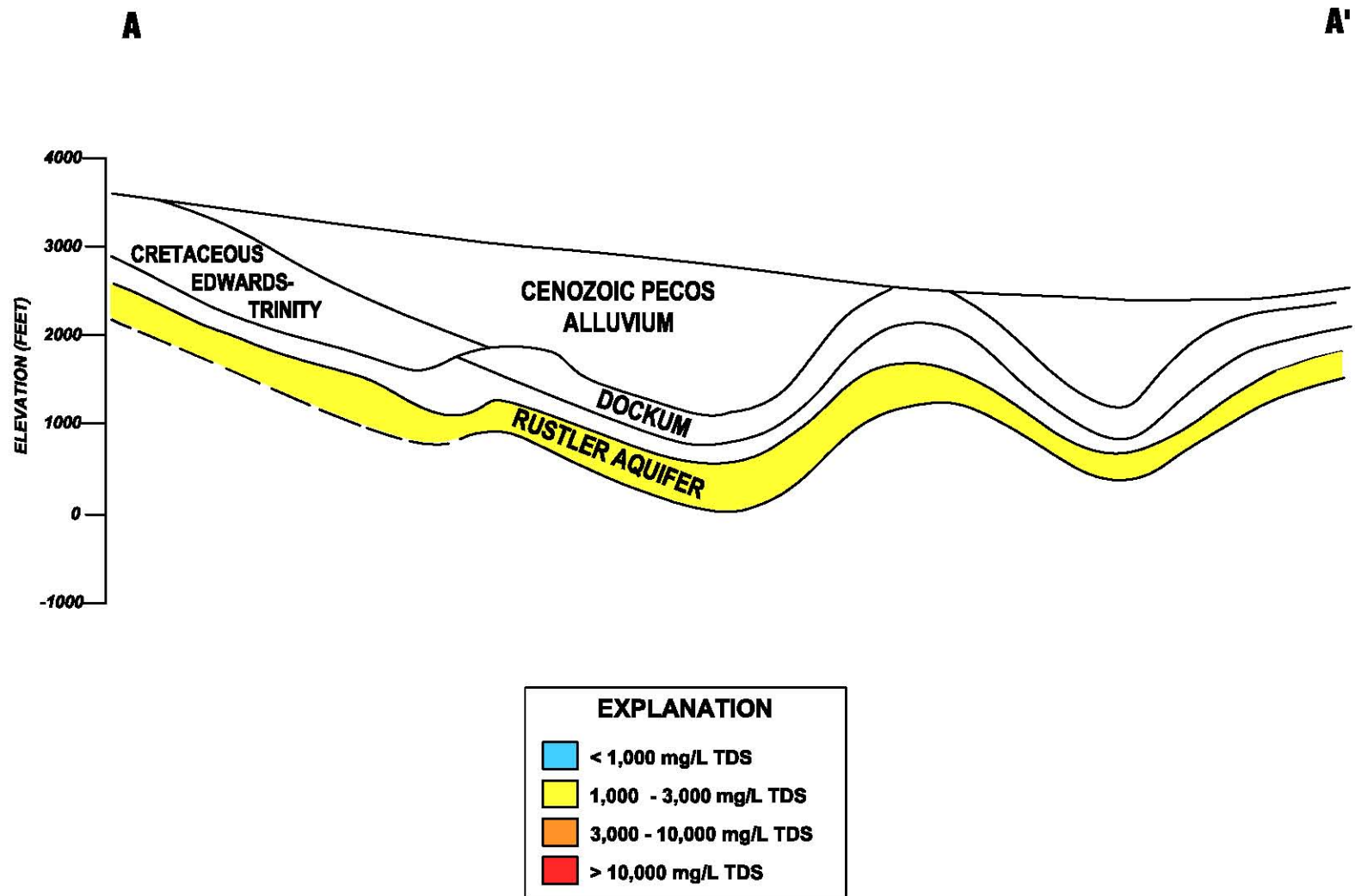
SIMPLIFIED CROSS SECTION OF THE RUSTLER AQUIFER WITH GENERALIZED WATER QUALITY RANGES (Modified from Ashworth, 1990)
