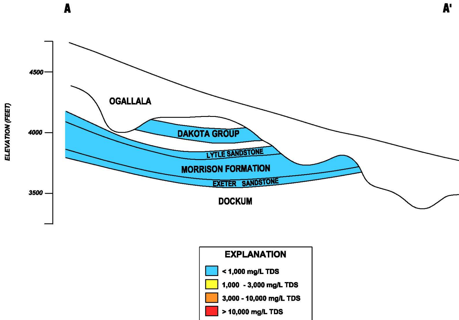
SIMPLIFIED CROSS SECTION OF THE RITA BLANCA AQUIFER WITH GENERALIZED WATER QUALITY RANGES
