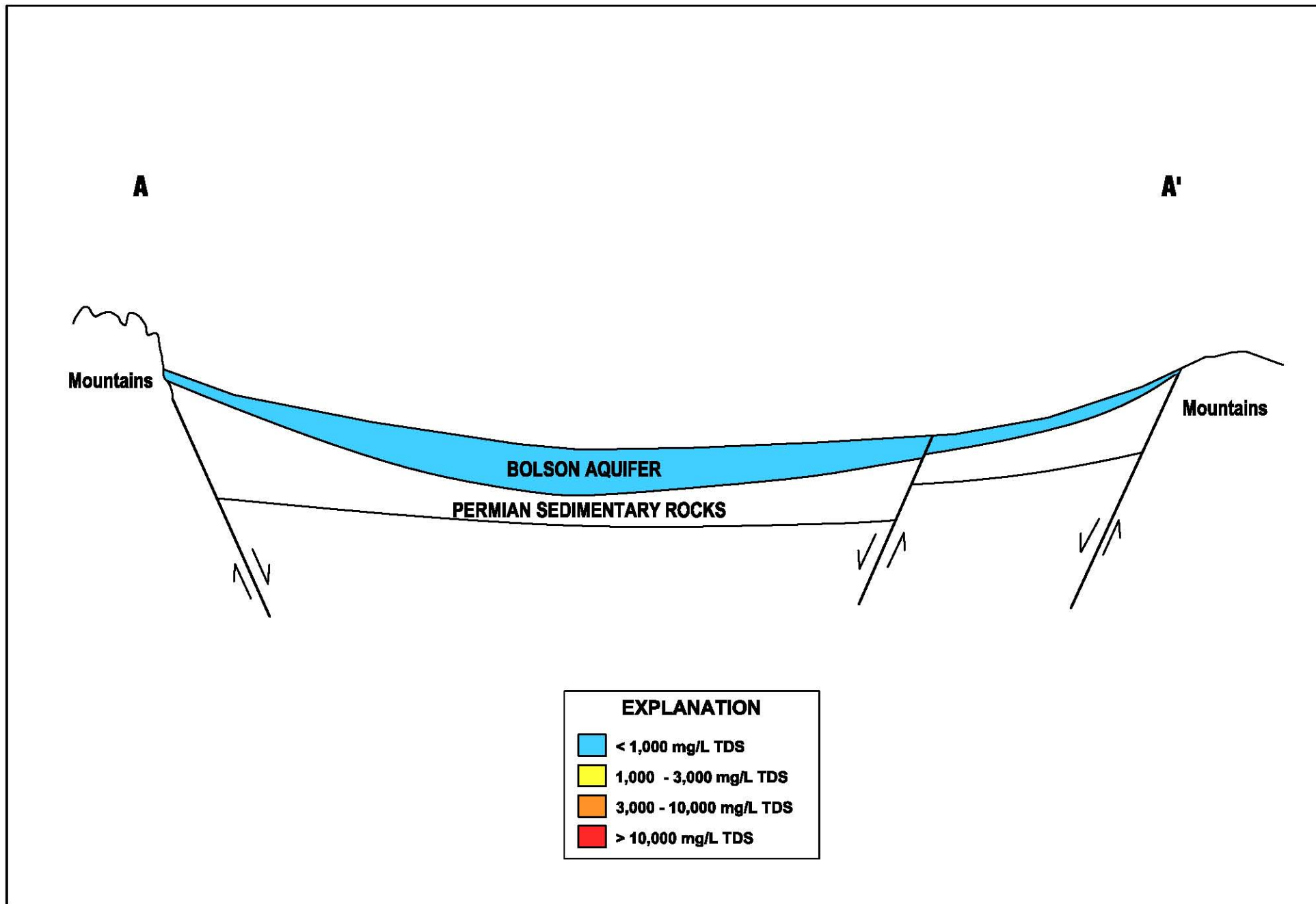
SIMPLIFIED CROSS SECTION OF THE WEST TEXAS BOLSONS AQUIFERS WITH GENERALIZED WATER QUALITY RANGES (Modified from Black, 1993)
